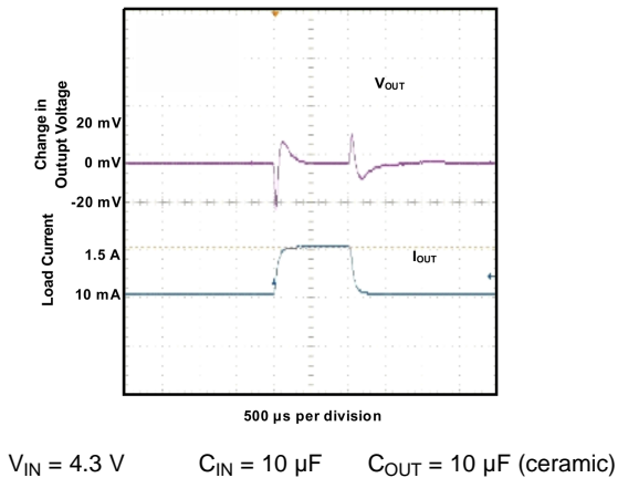
Figure 22. Load Transient Response
