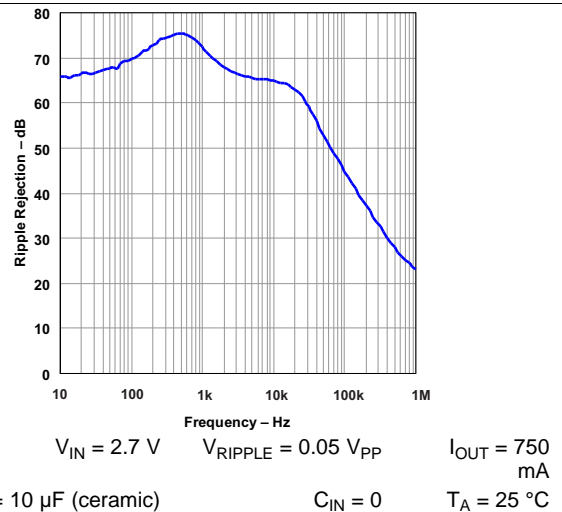
Figure 18. Ripple Rejection vs Frequency
